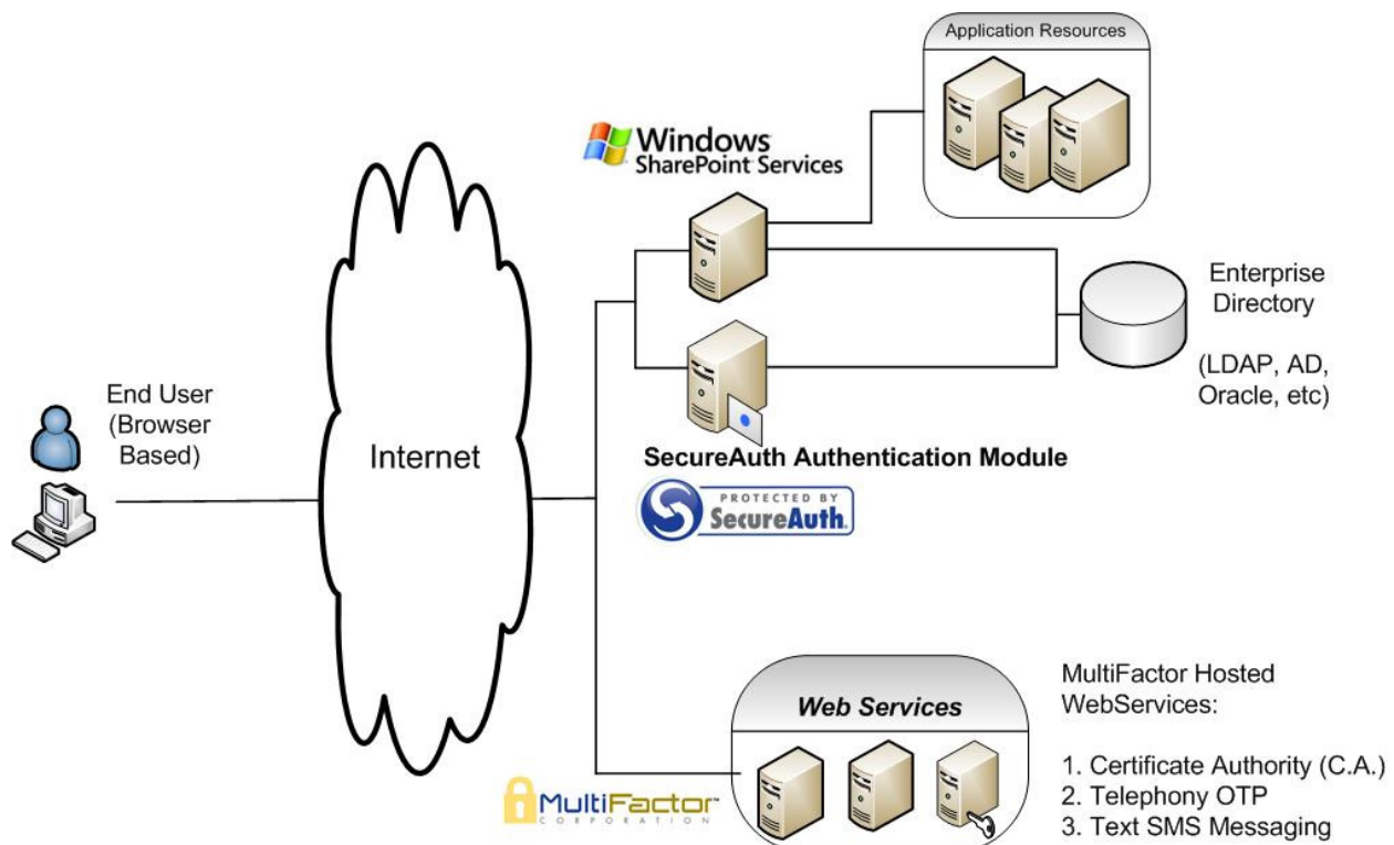
Figure 1 –SecureAuth® Integration into a Microsoft SharePoint Deployment
